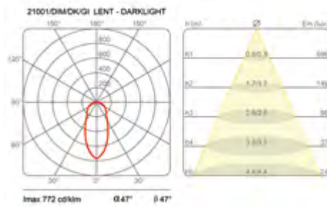
LAMPADA CON SCHERMO DARK-LIGHT (B) LAMP WITH DARK-LIGHT SCREEN
